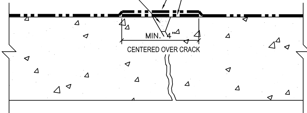
STRUCTURAL CRACKS w/< 1/16" MOVEMENT
