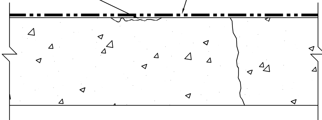
ROUGH CONCRETE AND NON-MOVING SHRINKAGE CRACKS
